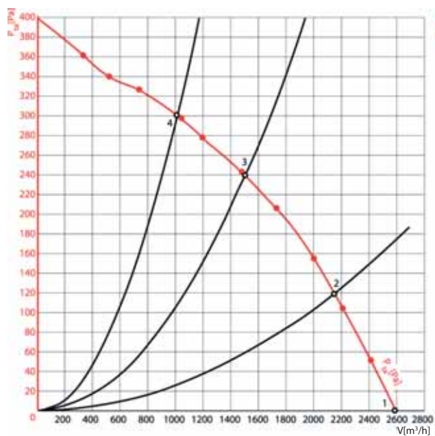
BKH 60-30/35-4D (380B)
